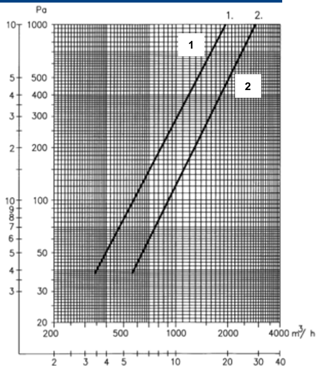
Graph 1. Air flow characteristics measured with air at 20 °C corresponding to air density of 1.20 kg/m 3 .
