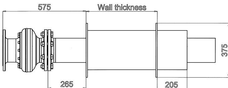
PVD-150 Exhaust Blast Valve dimensions
